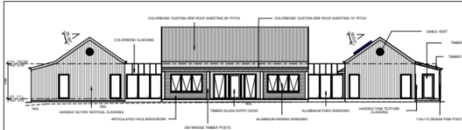
NORTH EAST ELEVATION (FRONT)
