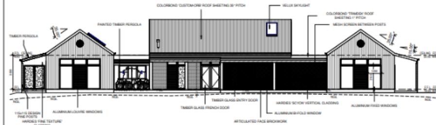
SOUTH WEST ELEVATION (REAR)
