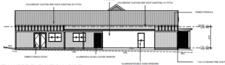
NORTH WEST ELEVATION (SIDE)
